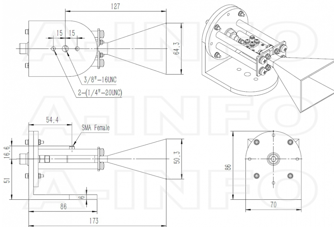
SMA-Female Output with L Type Mounting Bracket (Option, P/N: LB-42-10-C-MBL)
