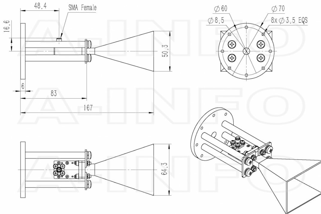
SMA-Female Output with Round Mounting Bracket (Option, P/N: LB-42-10-C-MB)
