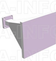
LB-42-20-ASPO Standard Gain Horn Antenna 18-26.5GHz 20dB Gain Rectangular Waveguide Interface
